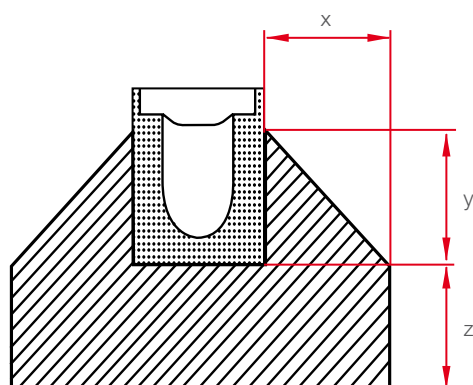
fig.b Key: x,y and z dimension of additional support.
