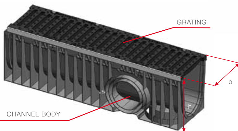
fig.d Key: h, b: internal dimensions (wetted perimeter).
